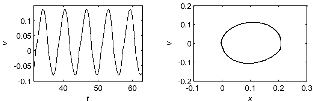
Figure 16. The time history of the velocity and phase portrait, where A = 8 \times 10^{-4} m .
